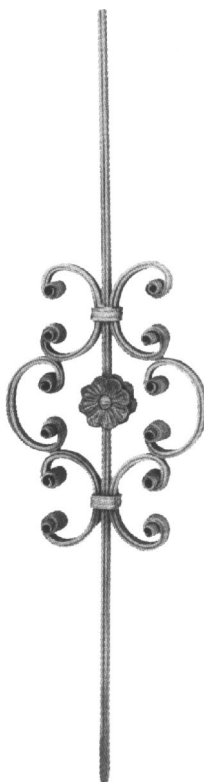
21.093.12 Baza: 12x12mm H: 900mm L: 230mm Canelat
